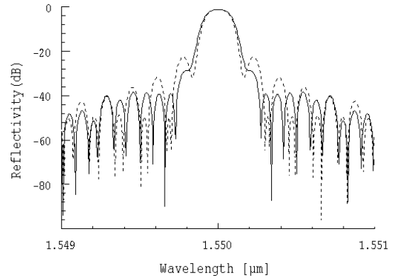
Figure 4: Reflectivity spectra for segmented Gaussian apodized normal FBGs with maximum error of 0.014 (solid line) and 0.08 (dashed line).
