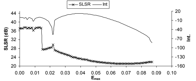
Figure 3: The SLSR and integration of error for the approximated Gaussian apodized FBGs as a function of error.
