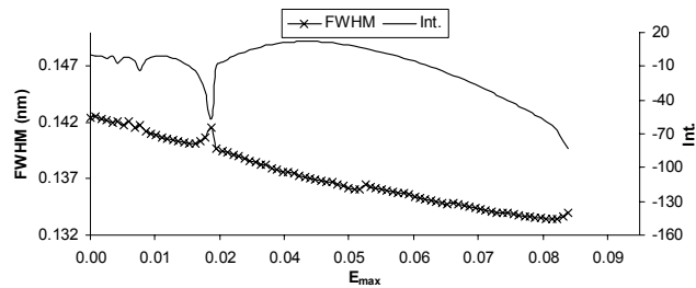
Figure 5: The approximated Gaussian apodized FBGs FWHM bandwidth and the integration of error as a function of maximum error.
