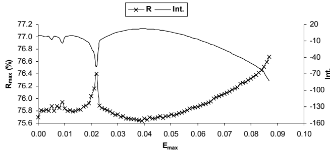
Figure 2: The maximum reflectivity and the integration of the error as a function of maximum error for approximated Gaussian apodized FBGs
