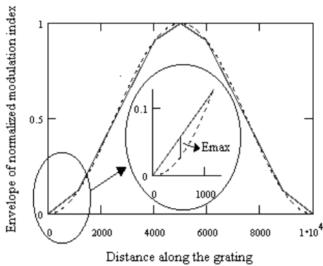
Figure 1: The error E_{max} of the segmented apodization profile
